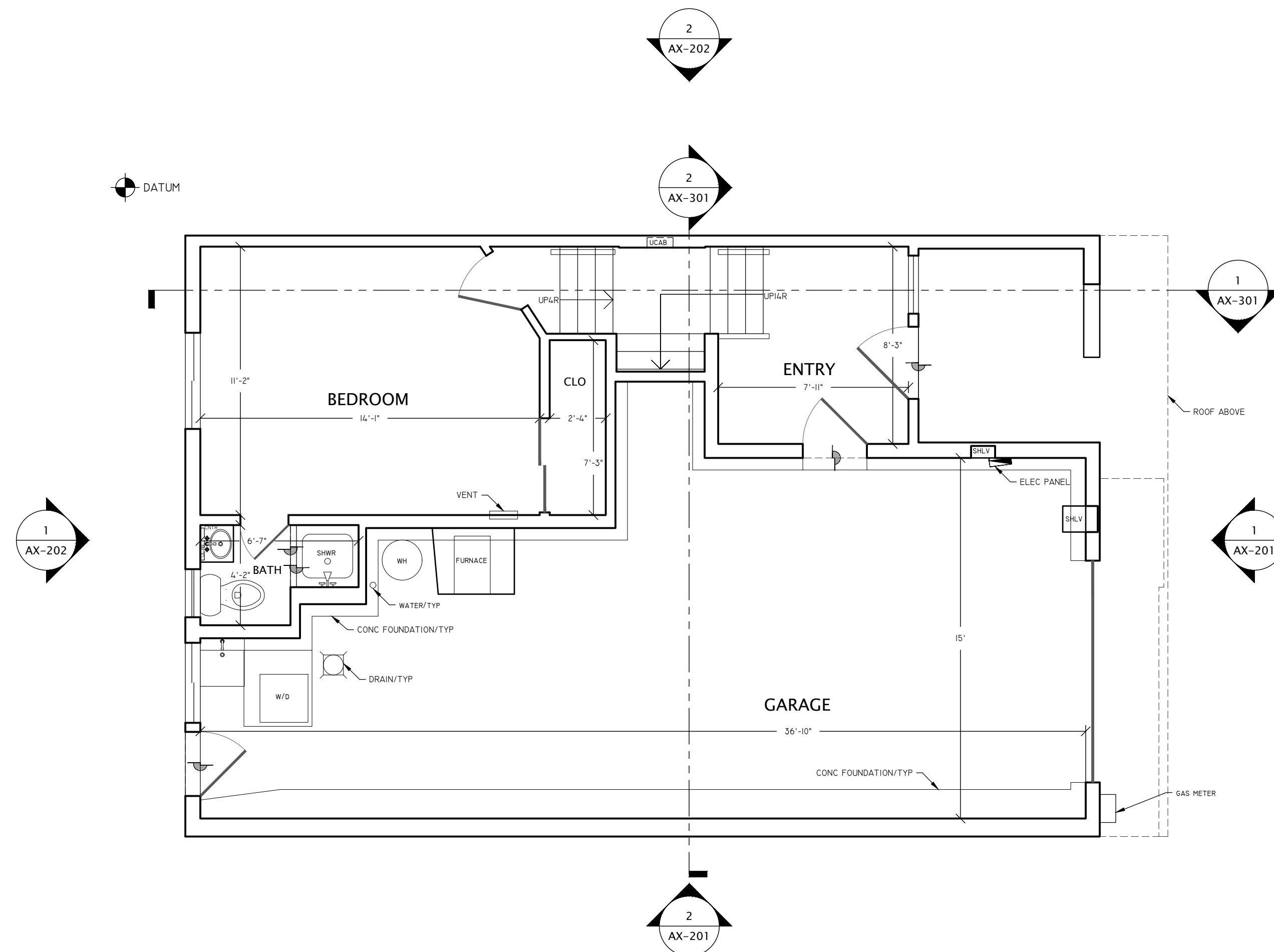
1 EXISTING ENTRY LEVEL FLOOR PLAN 891 SQFT GROSS MEASURED AREA 60 SQFT MEASURED EXTERIOR SURFACES
