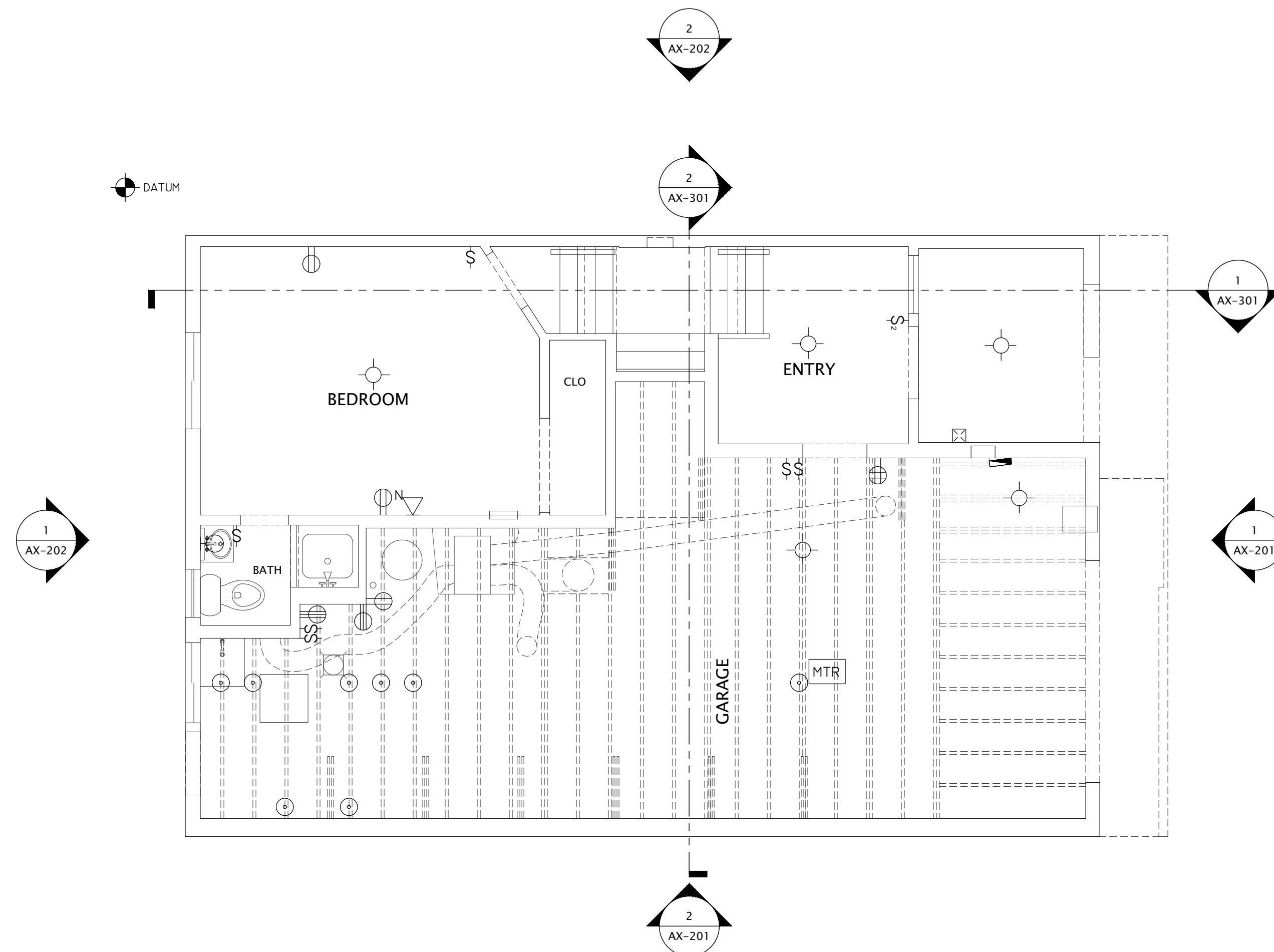
1 EXISTING ENTRY LEVEL ELECTRICAL & LIGHTING PLAN
