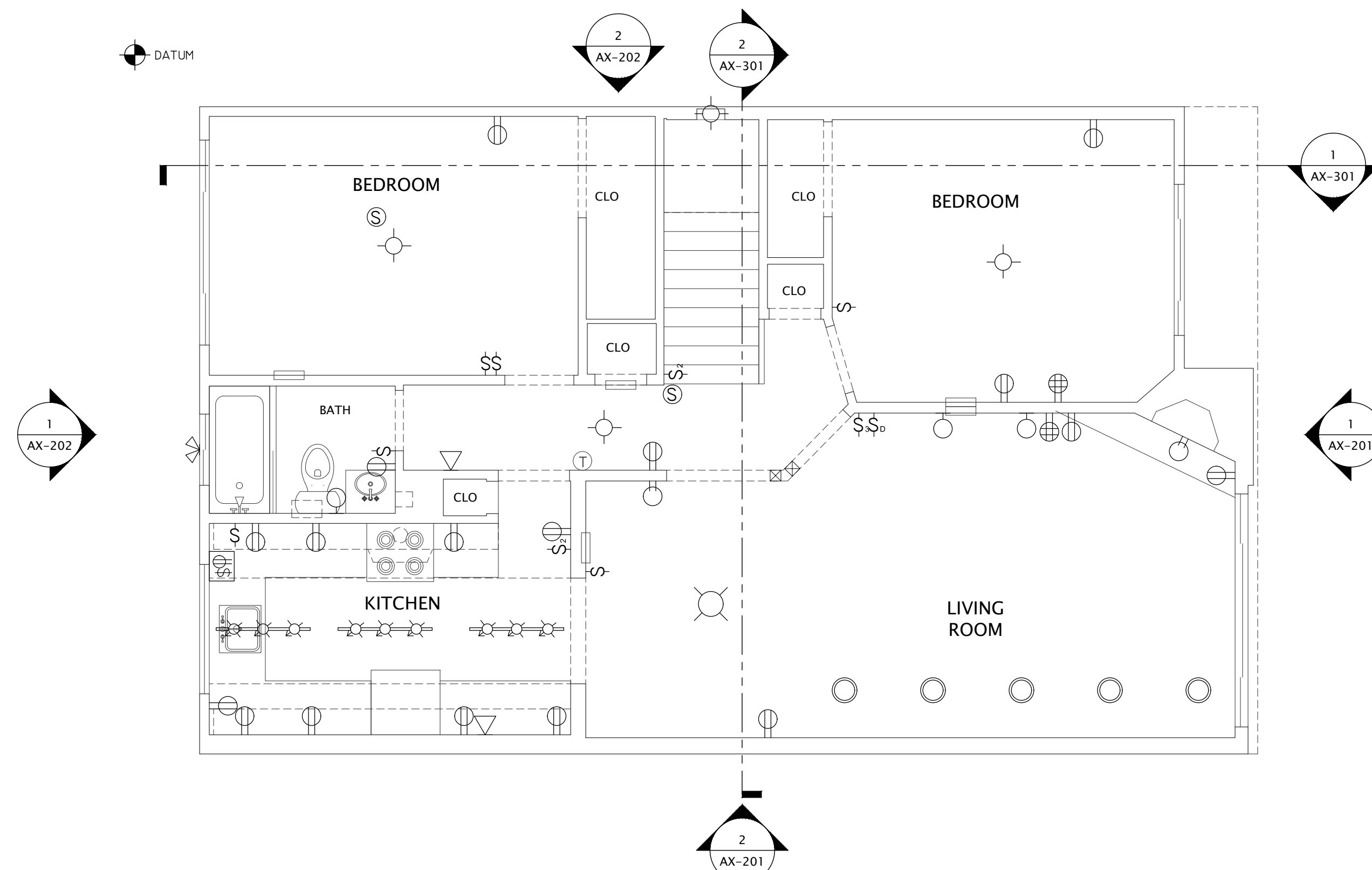
2 EXISTING SECOND LEVEL ELECTRICAL & LIGHTING PLAN
