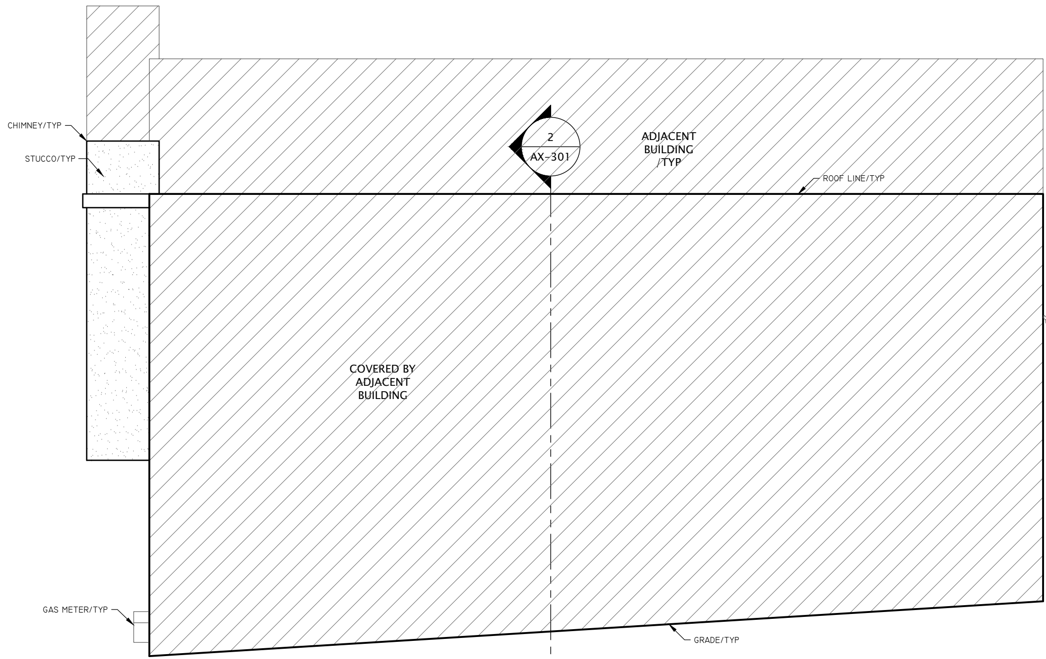
2 EXISTING NORTH ELEVATION
