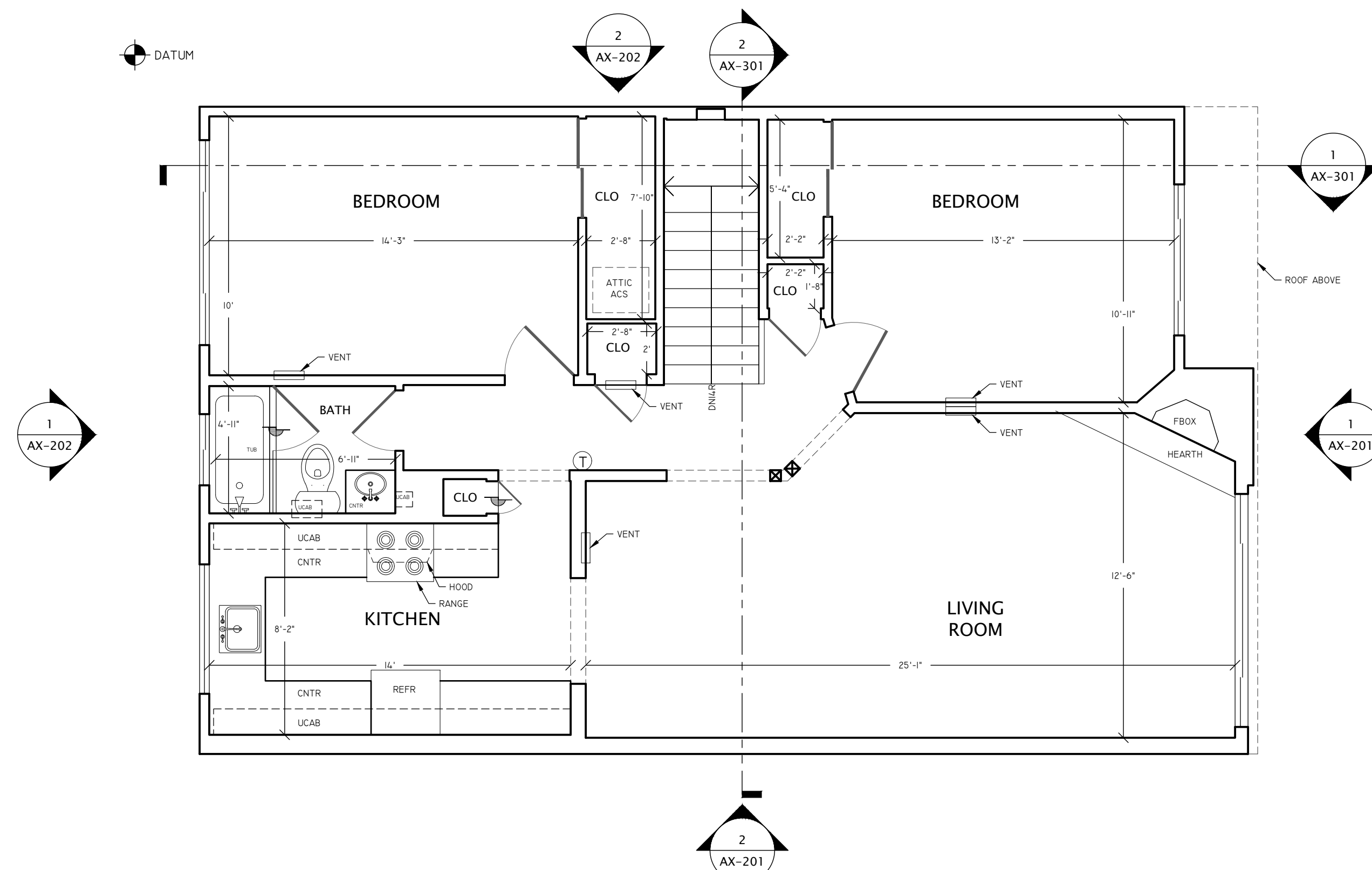
2 EXISTING SECOND LEVEL FLOOR PLAN 989 SQFT GROSS MEASURED AREA
