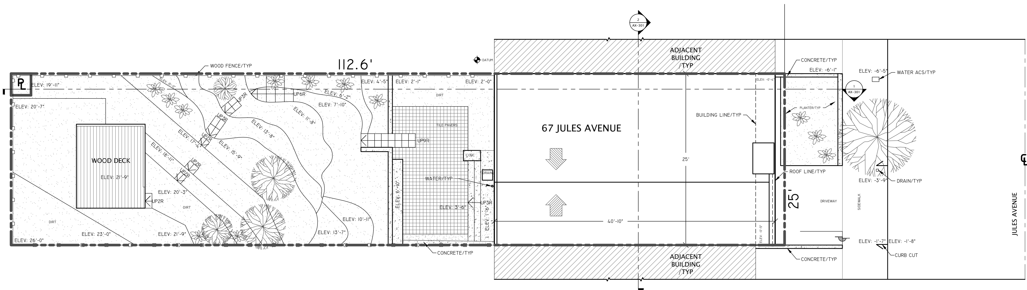
1 EXISTING LANDSCAPE SURVEY 2,815 SQFT (0.065 ACRE) SITE PLAN
