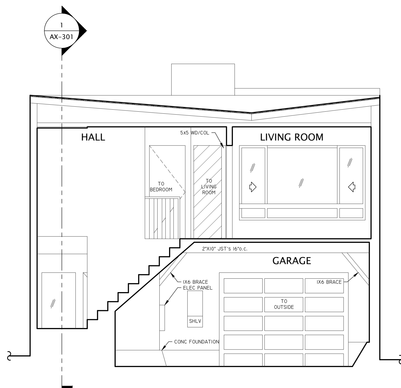
② EXISTING CROSS SECTION
